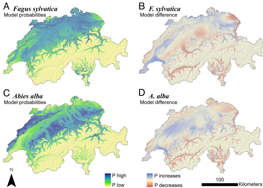
Fig. 5. Effect of adding climatic extremes on predicted spatial patterns. (A and C) Simulated probabilities of F. sylvatica (A) and A. alba (C) from GAMs using climatic means and extremes as predictors with no statistical interactions added. (B and D) The effect of adding extremes calculated as the difference between predicted probabilities of the more complex model using means and extremes and the model using means alone. Red and blue colors indicate the forcings of the standard deviations as predictors to decrease and increase the probabilities of the species models in A and C compared with the simple model consisting of climatic means alone.
