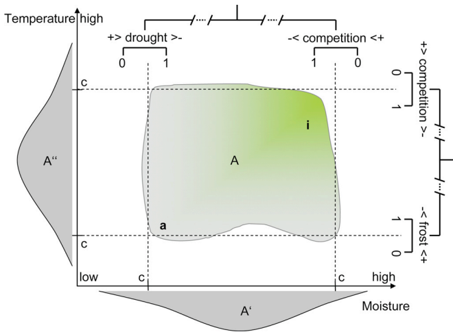
Fig. 1. Conceptual graph explaining possible effects of climatic and biotic constraints of species niches ( A ) with its effects on range limits along simple gradients of climatic means. The response shape typically fitted by regression-type models along gradients of mean climates is given as unimodal curves. Additionally, we illustrate the likely more local (with respect to ecological and spatial gradients) effect of extremes and biotic interactions as causal drivers of a reduction in the mean response along the same mean gradient. Zone a of the observed distribution in environmental space thus may represent areas where a species occurs close to the fundamental niche, whereas zone i does not give an indication of fundamental niche constraints, and the distribution may then be rather constrained by biotic interactions.
