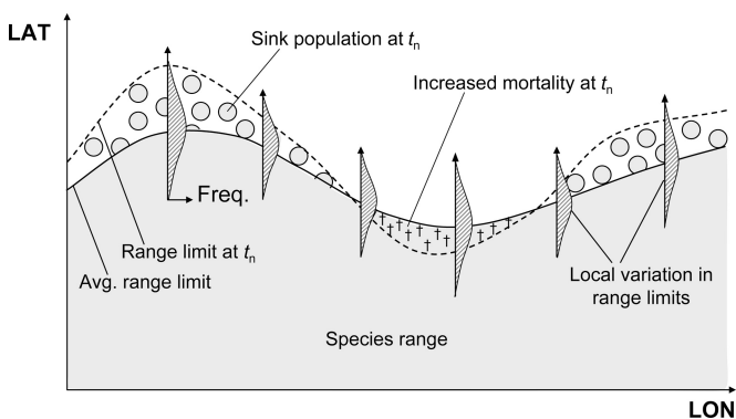
Fig. 6. Possible effects of climate variability at range margins. This graph illustrates that climatic means may sometimes explain the general range limit, whereas climatic extremes may rather influence local sink populations and extinctions ( t_n ). However, strong climatic variability at range margins may lead to asymmetric effects, and thus influence range limits additional to means.
