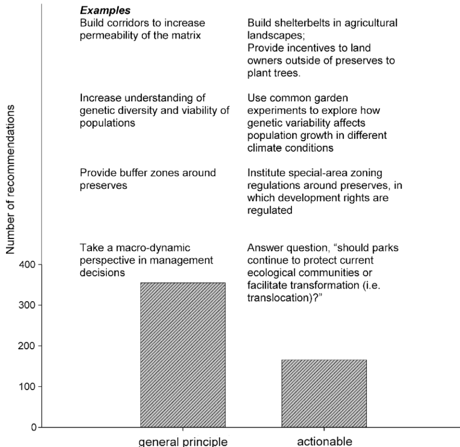
Fig. 1 – Examples and distribution of recommendations classified as “general principle” and “actionable”. Most recommendations offer general principles for climate change adaptation but lack specificity needed for implementation.
