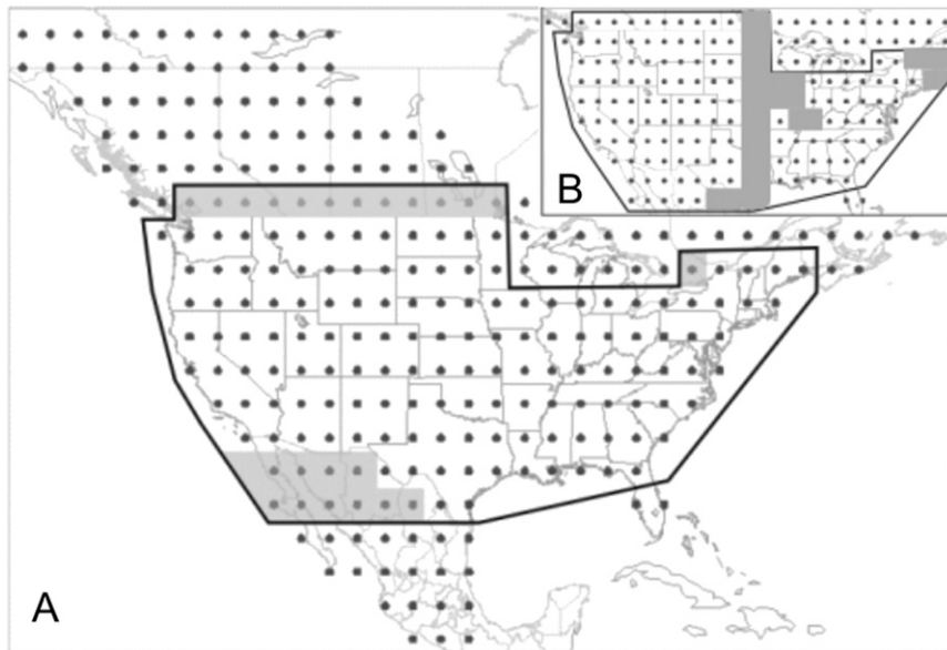
FIG. 1. PDSI grid points used in this study, based on a network of 286 points in a 2.5^{\circ} \times 2.5^{\circ} grid over North America for both instrumental and reconstructed data (updated from Cook et al. 2004; NOAA/National Climatic Data Center 2008a). Reconstruction data and methods are described in Cook et al. (2004) and associated online supporting materials. (a) Black outline indicates grid points with the common period 1404–2003, selected for the best spatial coverage over the longest period of time; gray shading indicates data points not used in the instrumental data analysis, 1900–2003 (data for non-U.S. points not available to 2003). (b) Inset shows grid points used for the 900–1350 analysis (outlined, nonshaded points).
