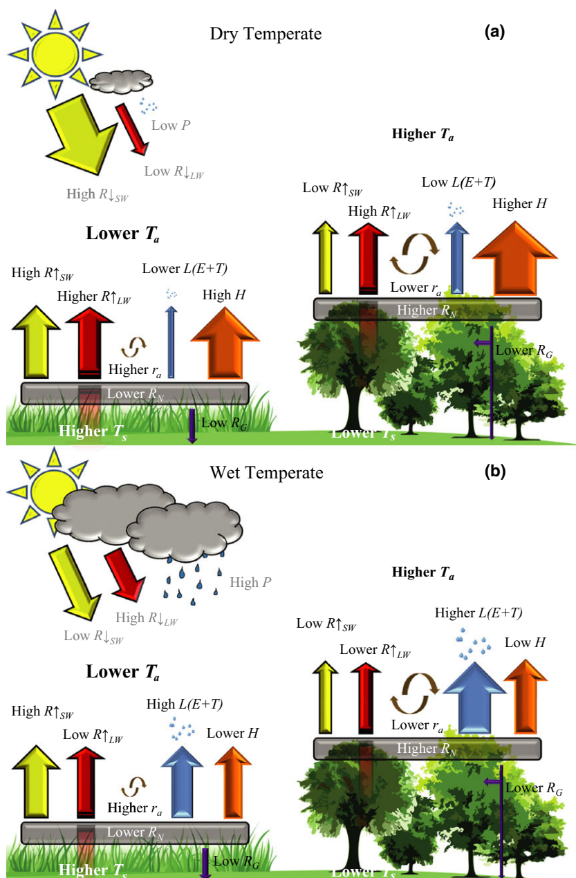
Fig. 1 Differences in the annual surface energy and moisture budgets between a temperate forest and an open grassland under dry (a) and wet (b) conditions. Horizontal fluxes of heat and moisture are excluded, and ' R_G ' includes heat stored by both the ground and vegetation. Although annual ' R_N ' is partitioned differently under arid and wet conditions, annual sensible heat fluxes (' H ') in temperate forests are typically higher relative to the grassland. ' T_a ' = air temperature; ' r_a ' = aerodynamic resistance.
