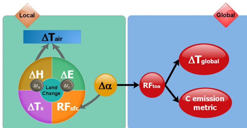
Fig. 3 Conceptual illustration of the relationships between the direct biogeophysical climate forcing mechanisms and corresponding metrics. ‘E’ = L(E + T) .
