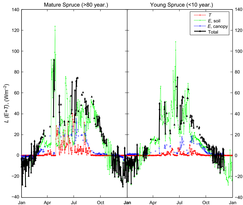
Fig. 2 Differences in the partitioning of daily E & T between adjacent young and mature spruce-dominant stands ( Picea abies (L.) H. Karst.) in eastern Norway during 2006. Adapted from Bright et al. (2014).
