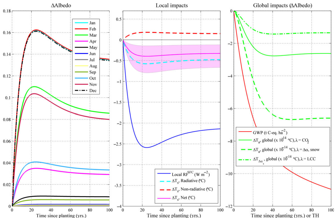
Fig. 5 Direct biogeophysical impacts of a change in tree species in boreal Norway. (Left) Changes in the monthly mean albedo when replacing spruce with birch over 100 years; (Middle) Local surface shortwave forcing (RF Δz s SFC ) and the local surface temperature response (ΔT s ; magenta curve) decomposed into radiative (dashed cyan) and nonradiative components (dashed red curve). ΔT s (t) is approximated with Eqn (16) based on the information presented in Table 6 and the ratio of annual mean radiative to nonradiative forcings. December and April net ΔT s make up the upper and lower ranges of the annual mean net ΔT s , respectively; (Right) Global impacts from the albedo changes.
