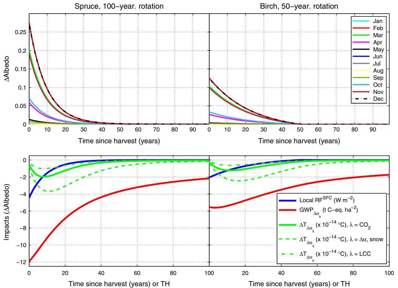
Fig. 4 (Upper panels) \Delta Albedo following a clear-cut harvest of typical spruce and birch stands in eastern Norway; (Lower panels) The associated climate impact as quantified with different metric alternatives. Three global mean temperature responses are presented: one using the equilibrium climate sensitivity ( \lambda ) for 2 \times CO_2 (Boucher & Reddy, 2008), a second for a 5% decrease in land snow albedo (Bellouin & Boucher, 2010), and a third for global historical LCC (Davin et al. , 2007).
